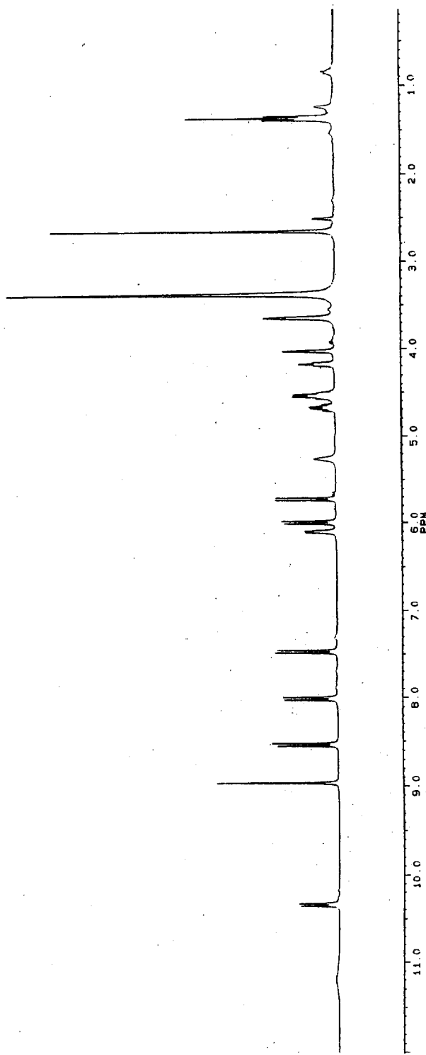
Figure S1. 1 H NMR spectrum of compound 2 (DMSO-d 6 , 300 MHz).
