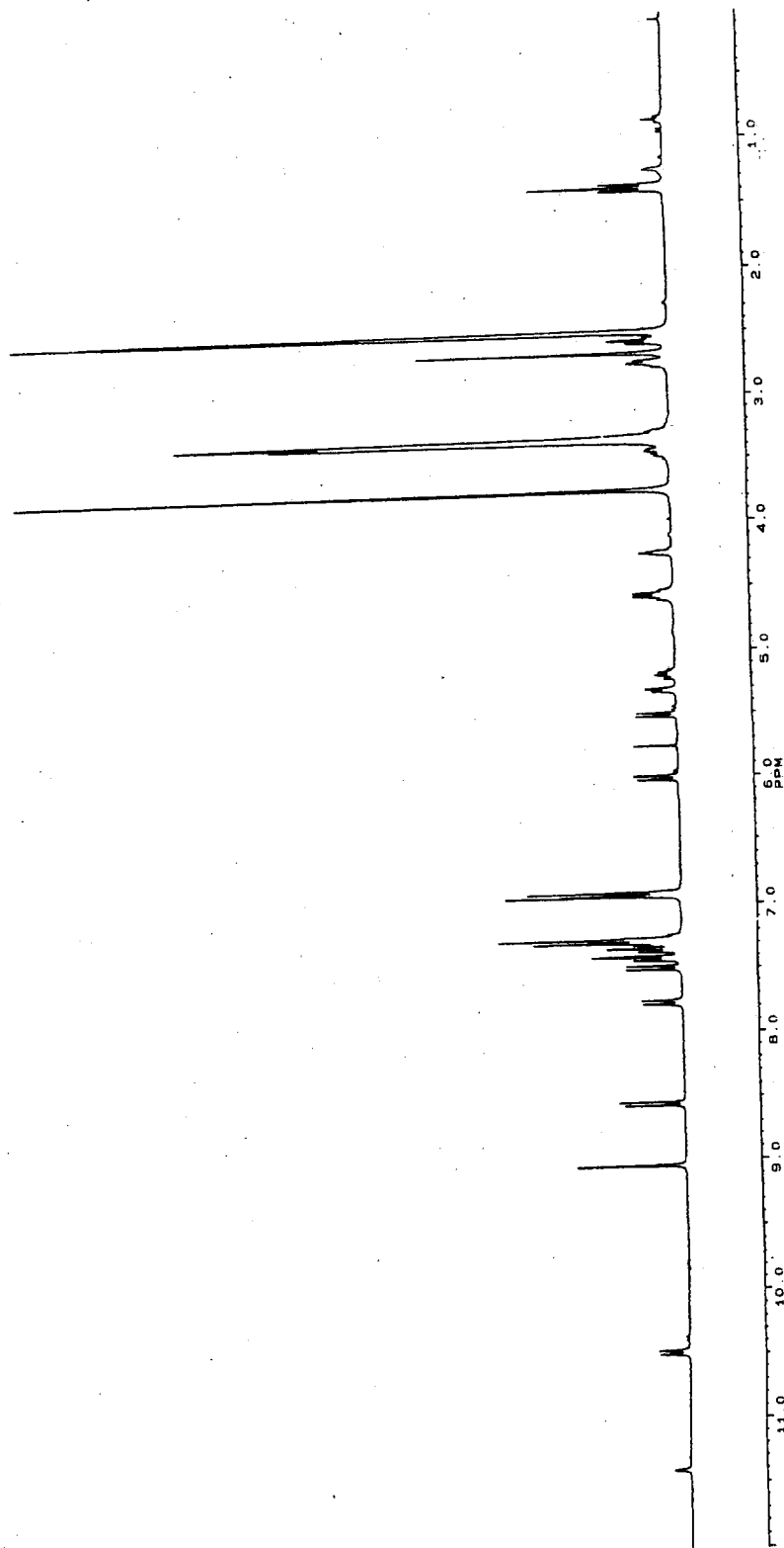
Figure S3. 1 H NMR spectrum of compound 4 (DMSO-d 6 , 300 MHz).
