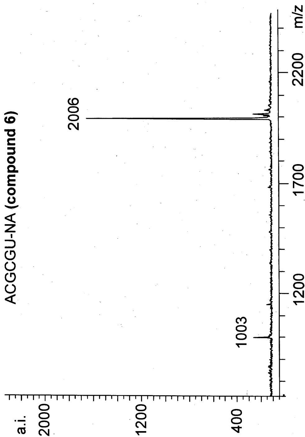
Figure S4. MALDI-TOF Mass Spectrum (linear, negative mode) of compound 6.
