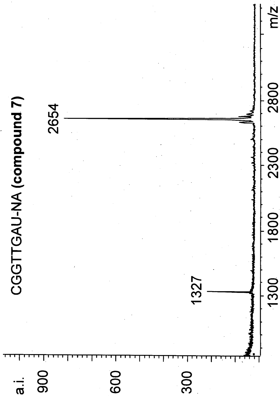
Figure S5. MALDI-TOF Mass Spectrum (linear, negative mode) of compound 7.
