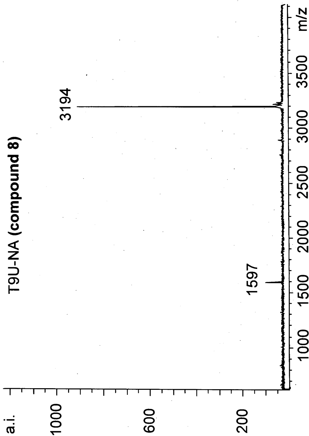
Figure S6. MALDI-TOF Mass Spectrum (linear, negative mode) of compound 8.
